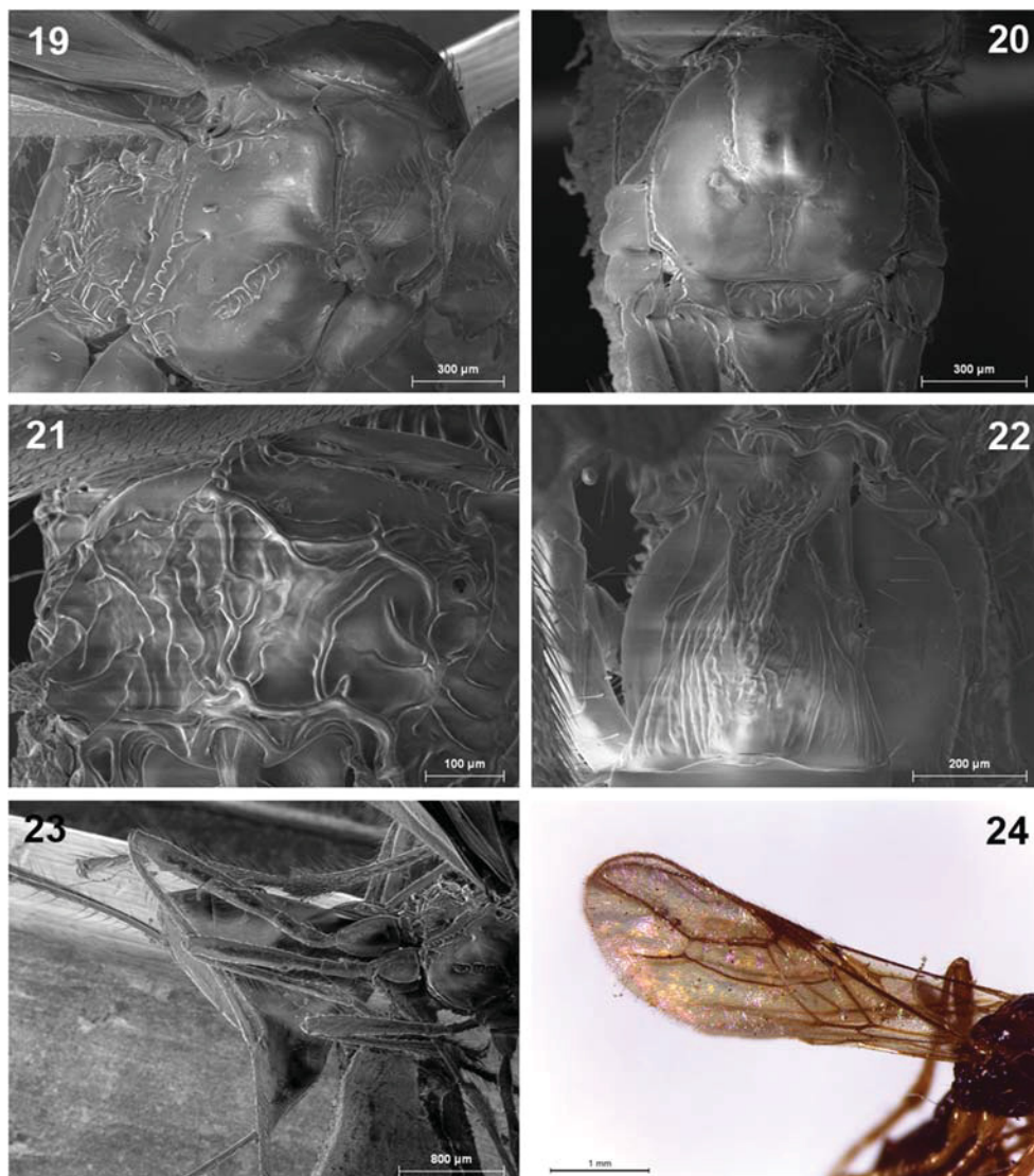
Figs 19–24. Asobara turneri Peris-Felipo sp. nov. (♀). 19 – mesosoma, lateral view; 20 – mesonotum; 21 – propodeum; 22 – first metasomal tergum; 23 – legs and metasoma, lateral view; 24 – fore wing.
